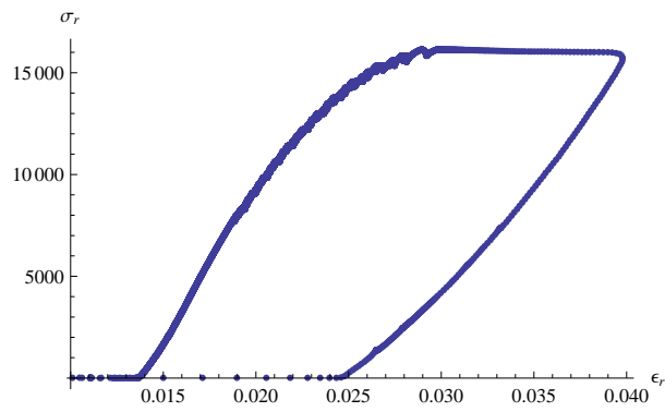
Figure A.54. Stress ( \sigma_r ) vs. strain ( \epsilon_r ) plot for test CG2-LP03
