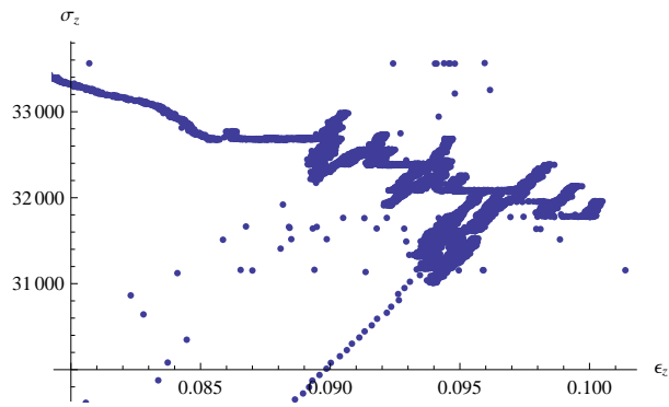
Figure A.21. The \sigma_z/\epsilon_z stress strain plot for test LP-TA22.
