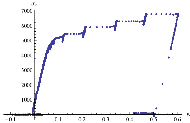
Figure A.20. The \sigma_r/\epsilon_r stress strain plot for test LP-TA22.
