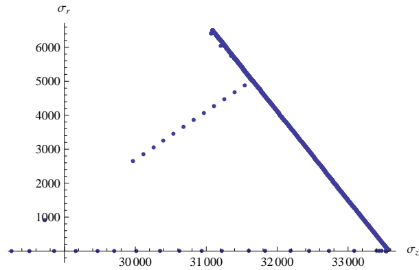
Figure A.38. The loading path for test LP-TA25 in r-z stress space
