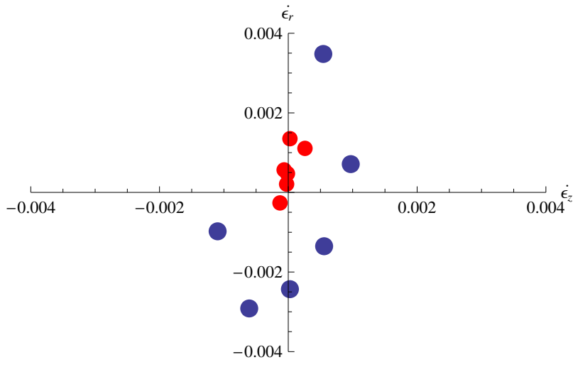
Figure A.25. Strain response envelope for the fifth loading cycle for test LP-TA22.
