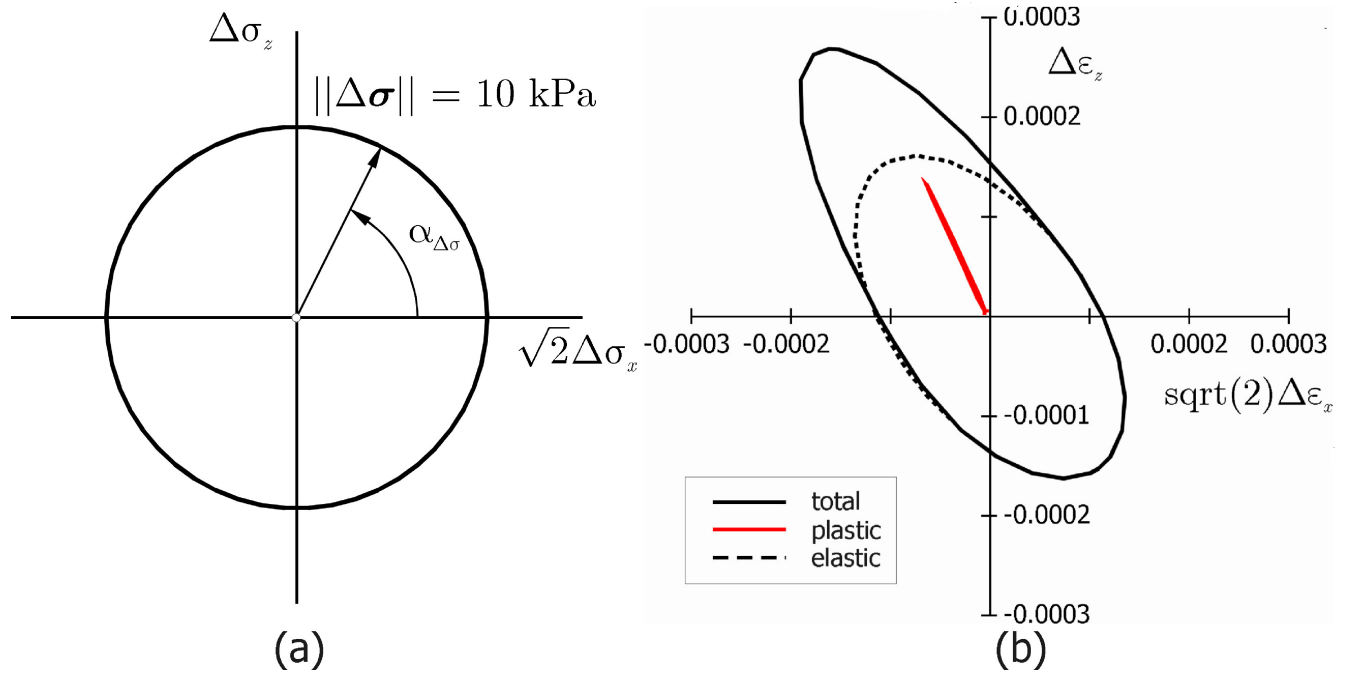
Figure 2.3. Results of Tamagnini’s DEM stress probe simulations. A set of axisymmetric stress increments represented by a unit circle in stress space (left), and the resulting strain increments mapped to strain space (right).
