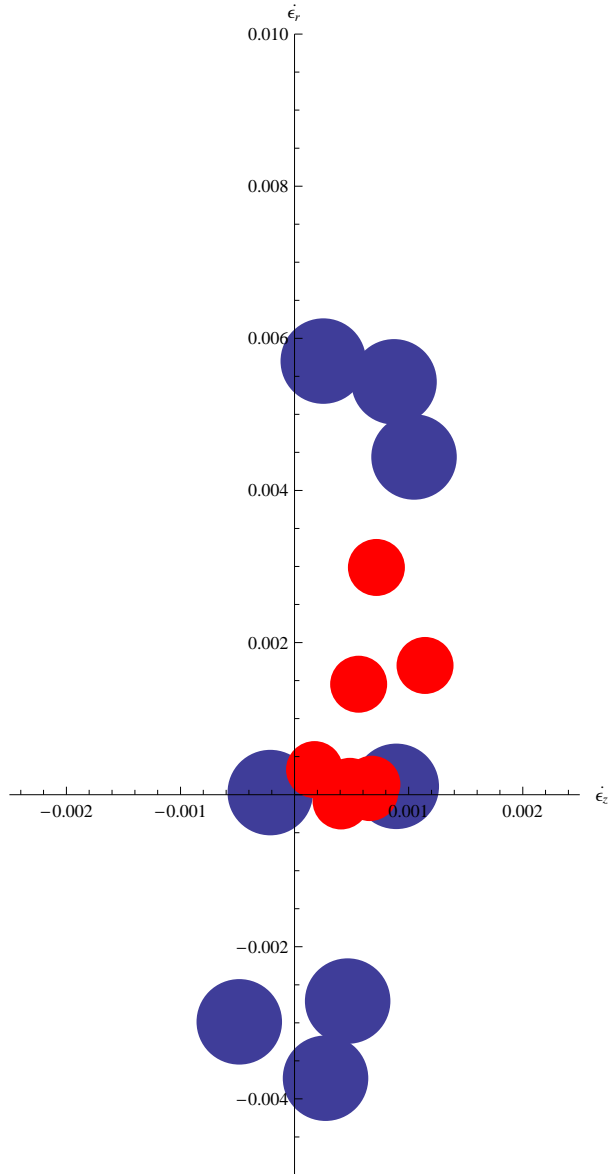
Figure A.35. Strain response envelope for the second loading cycle for test LP-TA24.
