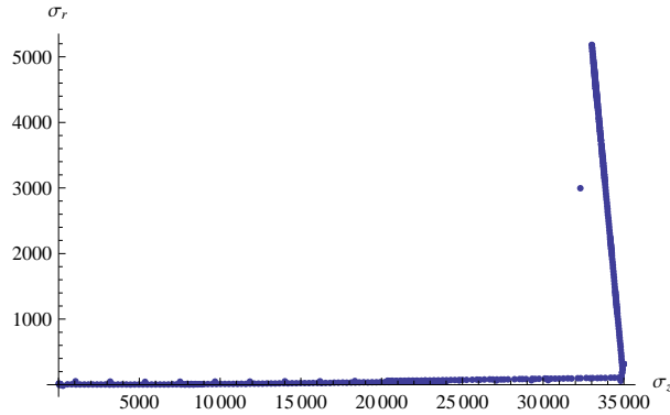
Figure A.6. The loading path for test LP-TA18 in r-z stress space
