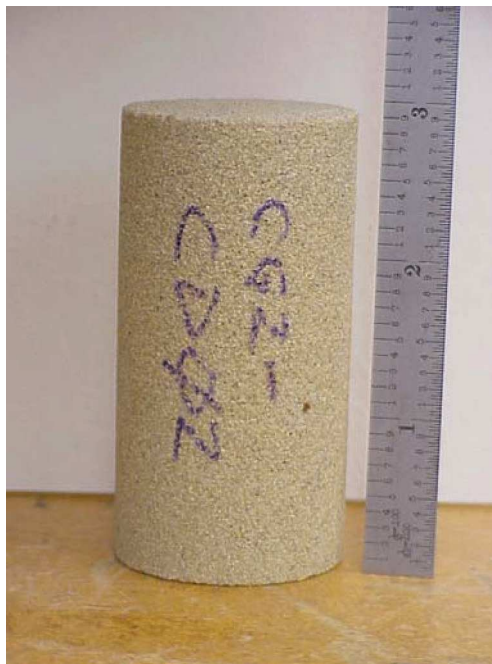
Figure 5.2. Right circular cylinder of Castlegate sandstone.
