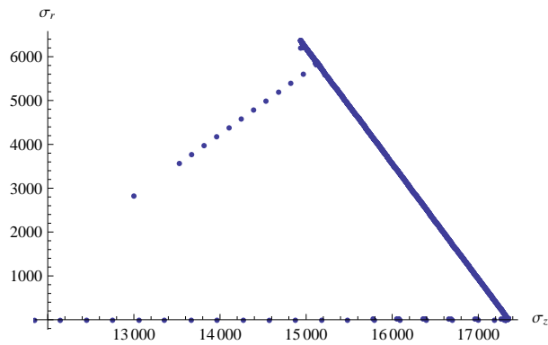
Figure A.41. The loading path for test LP-TA26 in r-z stress space
