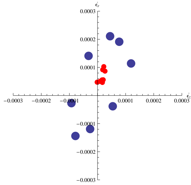
Figure A.62. Strain response envelope for the eighth loading cycle of test CG2-LP03.
