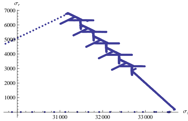
Figure A.19. The loading path for test LP-TA22 in r-z stress space
