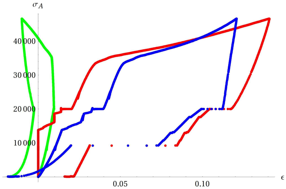
Figure A.4. Various strain measurements vs. axial stress for test CG2-CD10. Red curve is the axial strain, blue is the volumetric strain, and the green is the lateral strain.
