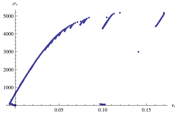
Figure A.7. The \sigma_r/\epsilon_r stress strain plot for test LP-TA18.
