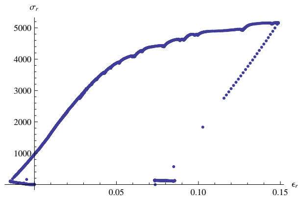
Figure 6.3. The \sigma_r vs. \epsilon_r stress strain curve for test LP-TA20, illustrating the initial anisotropy in the material. The anisotropy is evidenced by the change (decrease) in the strain \epsilon_r during the initial hydrostatic loading leg of the test where the \sigma_r stress remains nearly constant. This indicates that the material is undergoing a shear deformation due to a purely hydrostatic loading.
