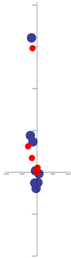
Figure A.49. Strain response envelope for the fourth loading cycle for test LP-TA27.
