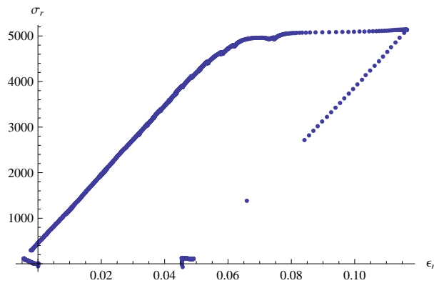
Figure A.10. The \sigma_r/\epsilon_r stress strain plot for test LP-TA19.
