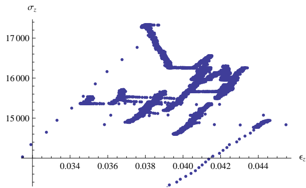
Figure A.46. The \sigma_z/\epsilon_z stress strain plot for test LP-TA27.
