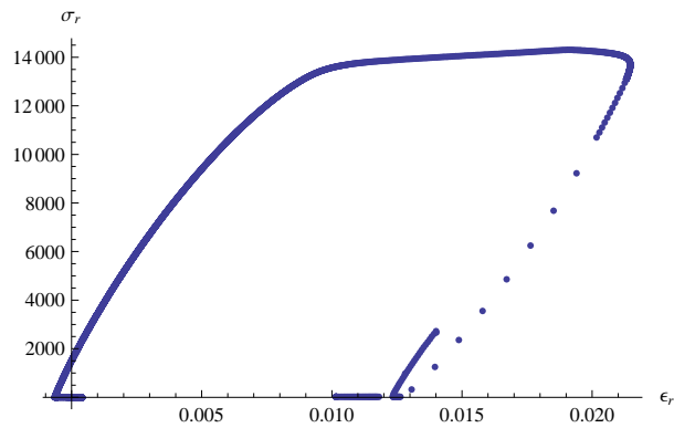
Figure A.51. Stress ( \sigma_r ) vs. strain ( \epsilon_r ) plot for test CG2-LP02
