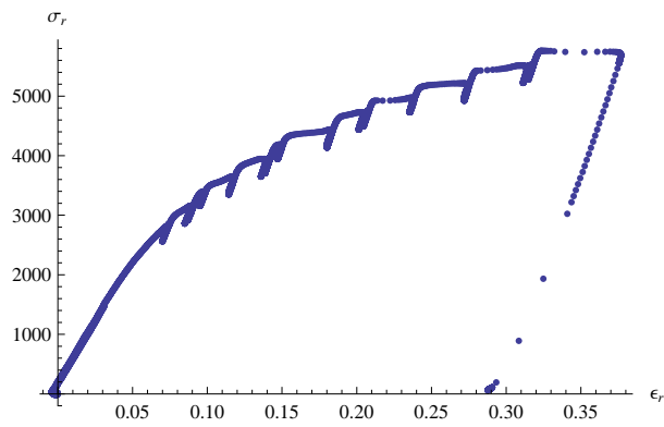
Figure A.27. The \sigma_r/\epsilon_r stress strain plot for test LP-TA23.
