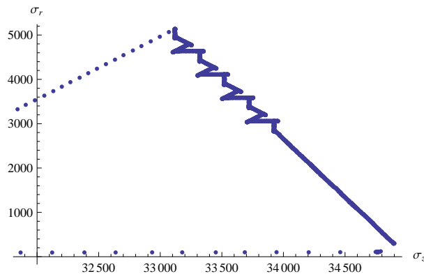
Figure A.9. The loading path for test LP-TA19 in r-z stress space
