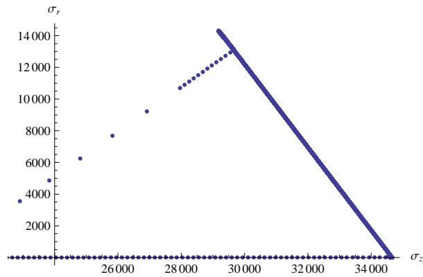
Figure A.50. The loading path used for test CG2-LP02
