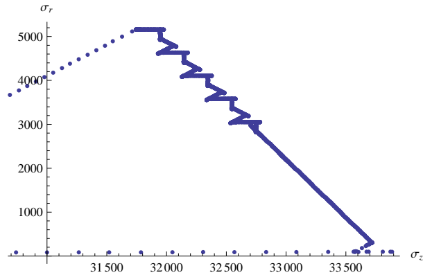
Figure A.13. The loading path for test LP-TA20 in r-z stress space
