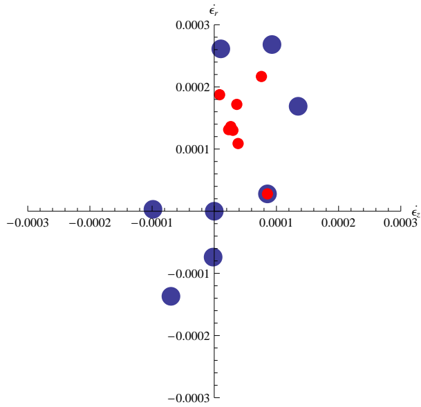
Figure A.65. Strain response envelope for the eleventh loading cycle of test CG2-LP03.
