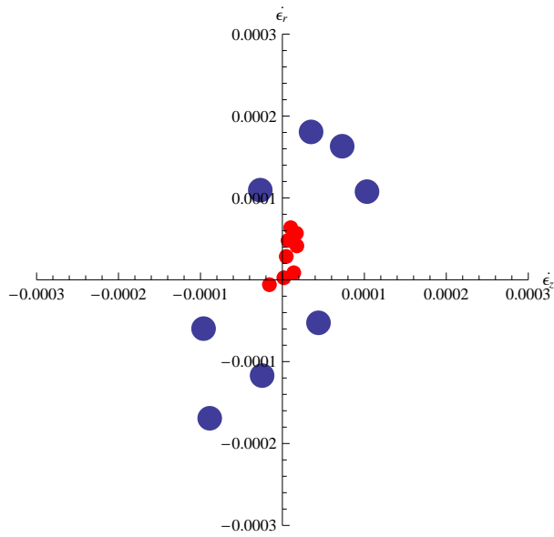
Figure A.58. Strain response envelope for the fourth loading cycle of test CG2-LP03.
