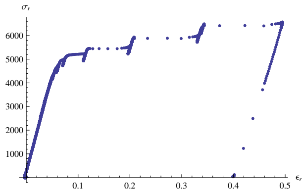
Figure A.45. The \sigma_r/\epsilon_r stress strain plot for test LP-TA27.
