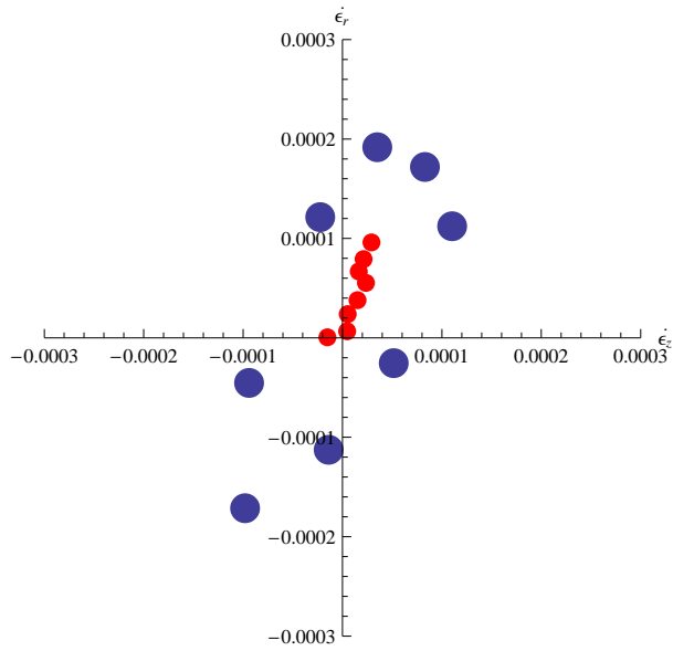
Figure A.59. Strain response envelope for the fifth loading cycle of test CG2-LP03.
