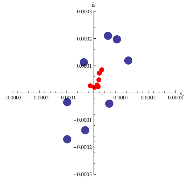
Figure A.61. Strain response envelope for the seventh loading cycle of test CG2-LP03.
