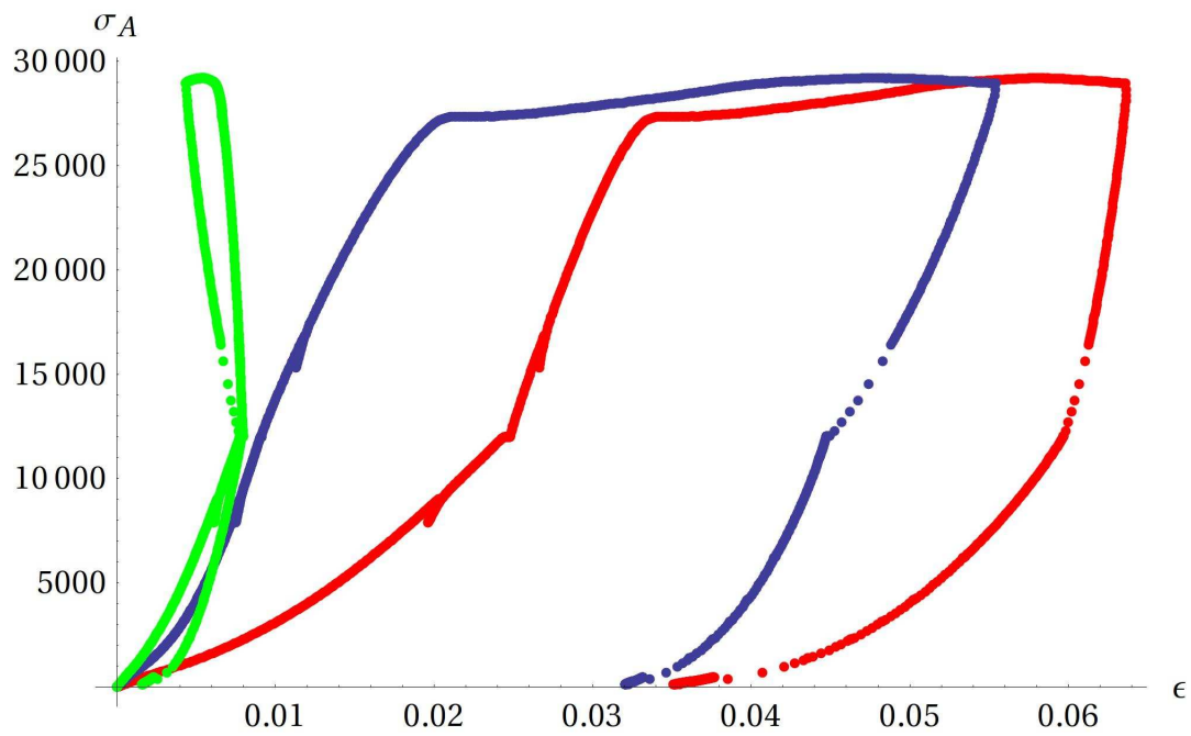
Figure A.5. Various strain measurements vs. axial stress for test CG2-CD11. Red curve is the axial strain, blue is the volumetric strain, and the green is the lateral strain.
