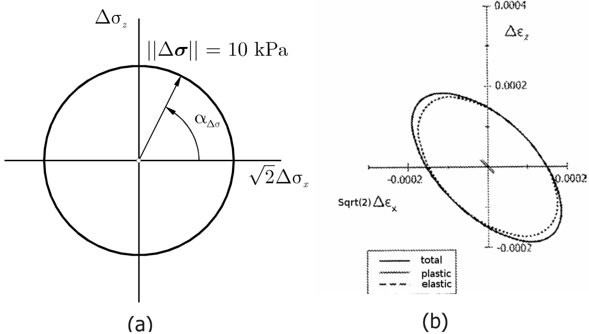
Figure 2.4. Strain response envelope for axisymmetric stress probes at stress state B' from Tamagnini's DEM simulations. (Courtesy of C. Tamagnini)
