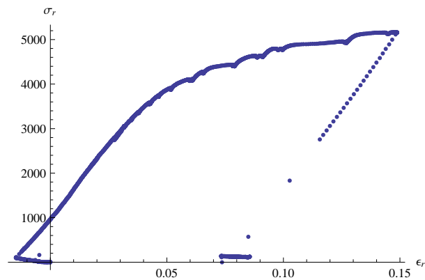
Figure A.14. The \sigma_r/\epsilon_r stress strain plot for test LP-TA20.
