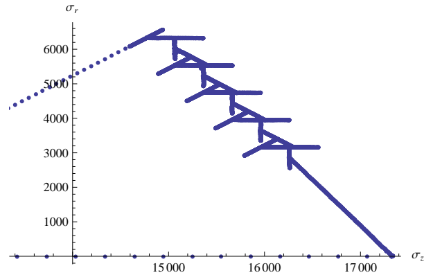
Figure A.44. The loading path for test LP-TA27 in r - z stress space
