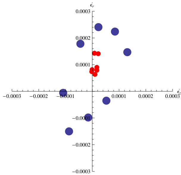
Figure A.64. Strain response envelope for the tenth loading cycle of test CG2-LP03.
