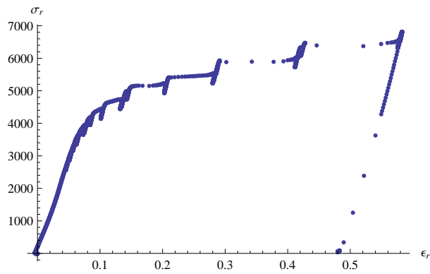
Figure A.33. The \sigma_r/\epsilon_r stress strain plot for test LP-TA24.
