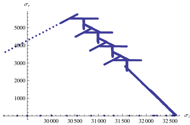
Figure A.26. The loading path for test LP-TA23 in r-z stress space
