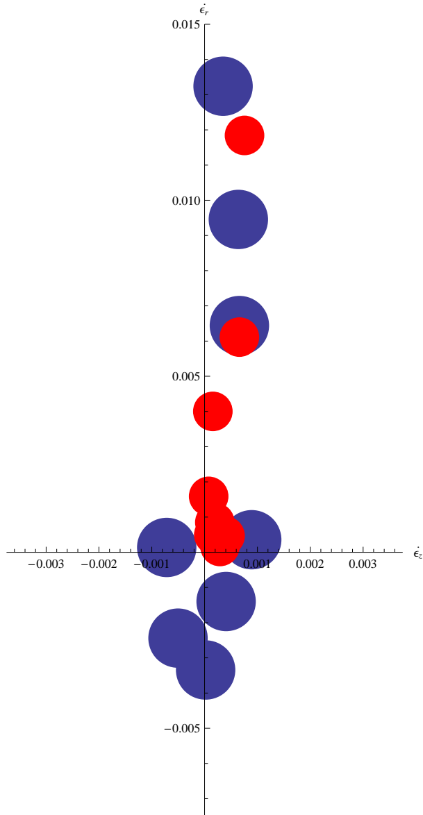
Figure A.36. Strain response envelope for the third loading cycle for test LP-TA24.
