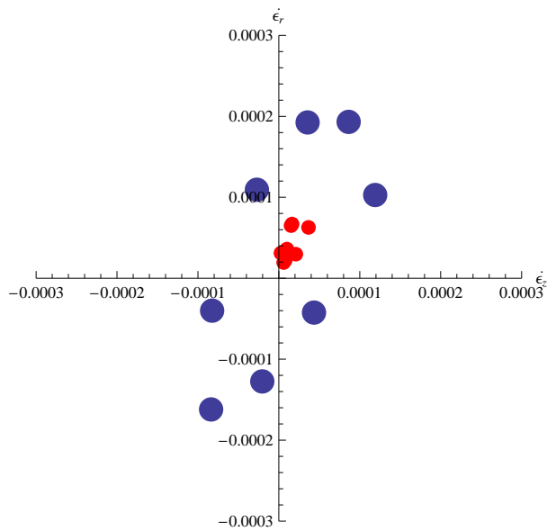
Figure A.60. Strain response envelope for the sixth loading cycle of test CG2-LP03.
