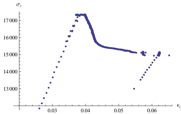
Figure A.43. The \sigma_z/\epsilon_z stress strain plot for test LP-TA26.
