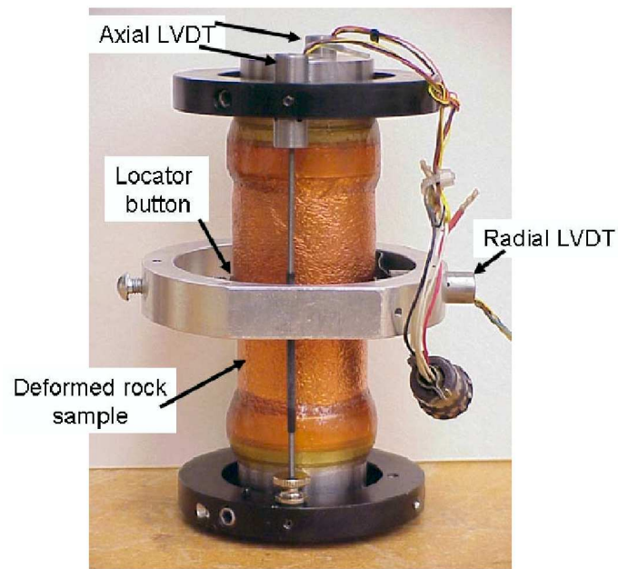
Figure 5.4. Right circular cylinder of deformed Castlegate sandstone, showing the complete sample assembly with axial and radial LVDTs
