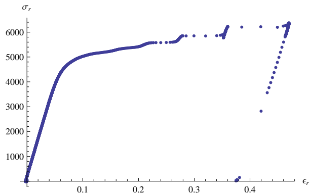
Figure A.42. The \sigma_r/\epsilon_r stress strain plot for test LP-TA26.
