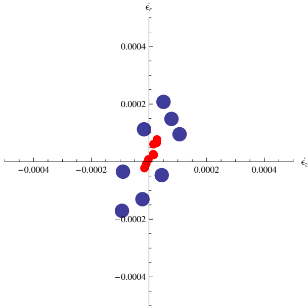
Figure A.56. Strain response envelope for the second loading cycle of test CG2-LP03.
