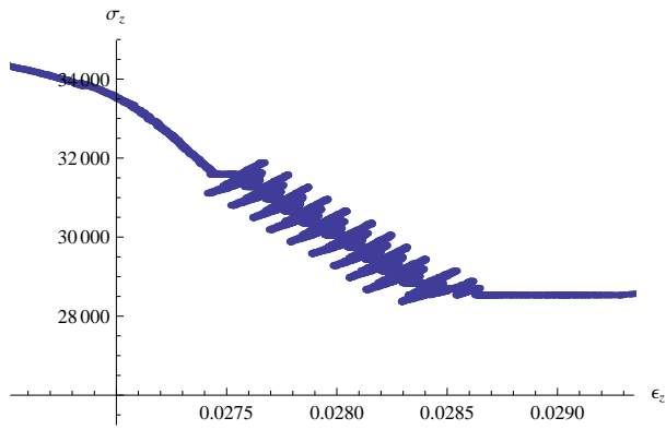
Figure A.55. Stress ( \sigma_z ) vs. strain ( \epsilon_z ) plot for test CG2-LP03
