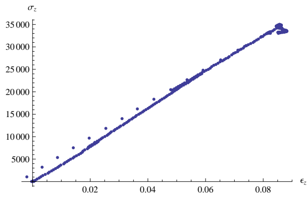
Figure A.8. The \sigma_z/\epsilon_z stress strain plot for test LP-TA18.
