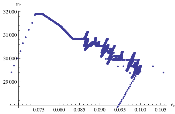
Figure A.34. The \sigma_z/\epsilon_z stress strain plot for test LP-TA24.
