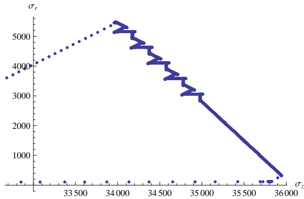
Figure A.16. The loading path for test LP-TA21 in r-z stress space
