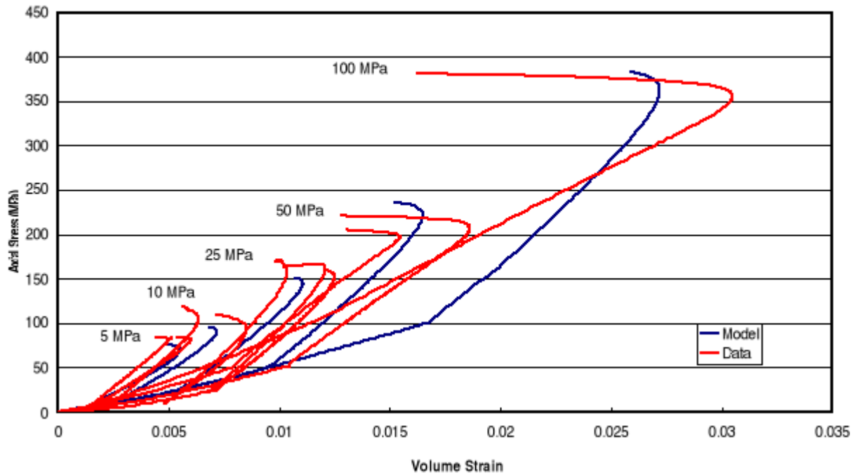
Figure 6.4. Validation of a geomechanics model for loading of Sidewinder Tuff under triaxial compression [2]. (Note: the present work aims to extend validation for changes in the loading direction away from standard triaxial compression load paths of this kind.)
