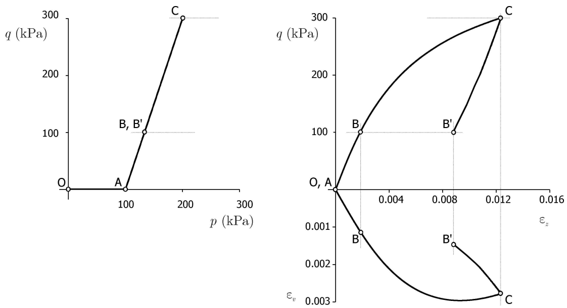
Figure 2.2. Triaxial compression load path used in DEM simulations performed by Tamagnini. Here q is the equivalent shear stress, and p is the mean stress. Also \epsilon_z is the strain in the z (axial)-direction, and \epsilon_v is the volumetric strain. The points at which stress probes were applied are labeled B and B' . (Courtesy of C. Tamagnini)
