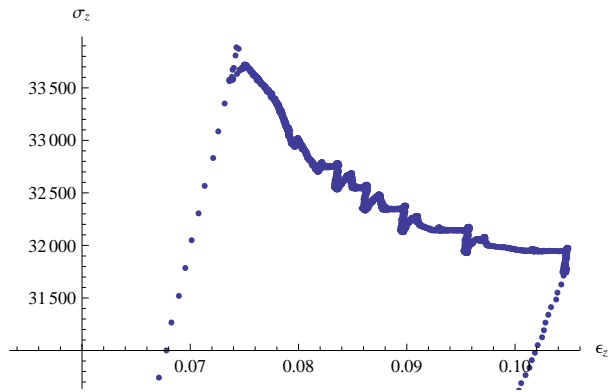
Figure A.15. The \sigma_z/\epsilon_z stress strain plot for test LP-TA20.
