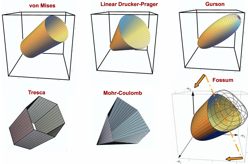
Figure 1.2. Common isotropic yield surfaces. Von Mises and Drucker-Prager models are often used for metals. Gurson’s function, and others like it, are used for porous media. Tresca and Mohr-Coulomb models approximate the yield threshold for brittle media. Fossium’s model, and others like it, combine these features to model realistic geological media.
