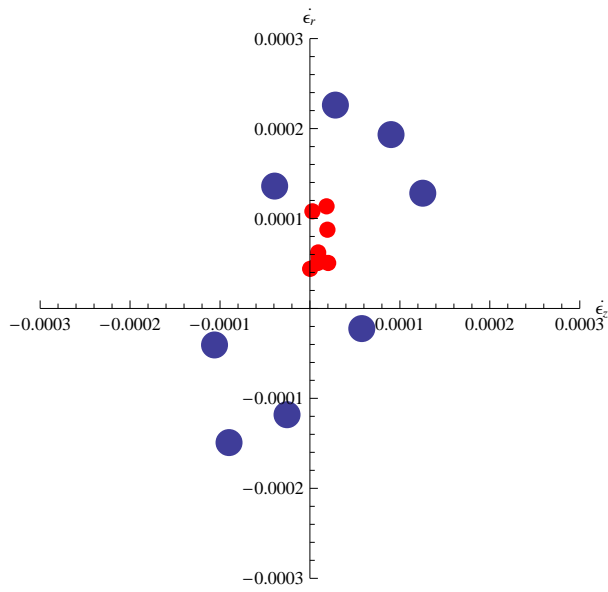
Figure A.63. Strain response envelope for the ninth loading cycle of test CG2-LP03.
