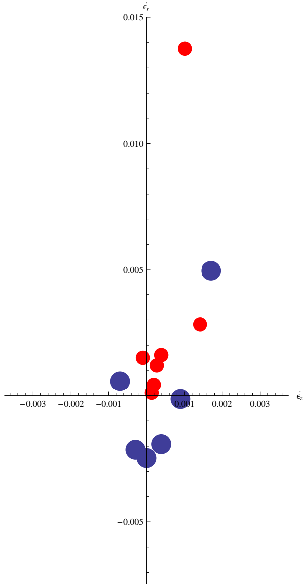
Figure A.30. Strain response envelope for the third loading cycle for test LP-TA23.
