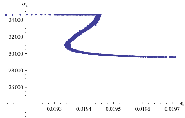
Figure A.52. Stress ( \sigma_z ) vs. strain ( \epsilon_z ) plot for test CG2-LP02
