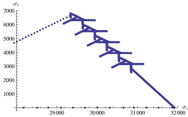
Figure A.32. The loading path for test LP-TA24 in r-z stress space
