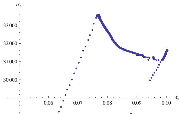
Figure A.40. The \sigma_z/\epsilon_z stress strain plot for test LP-TA25.
