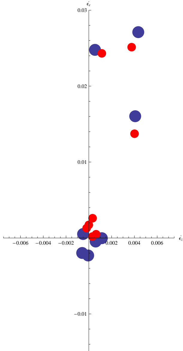
Figure A.31. Strain response envelope for the fourth loading cycle for test LP-TA23.
