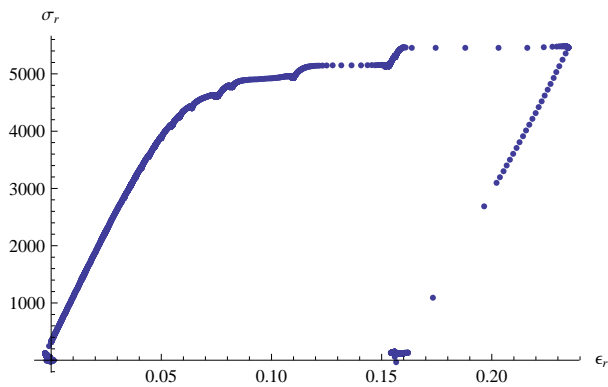
Figure A.17. The \sigma_r/\epsilon_r stress strain plot for test LP-TA21.
