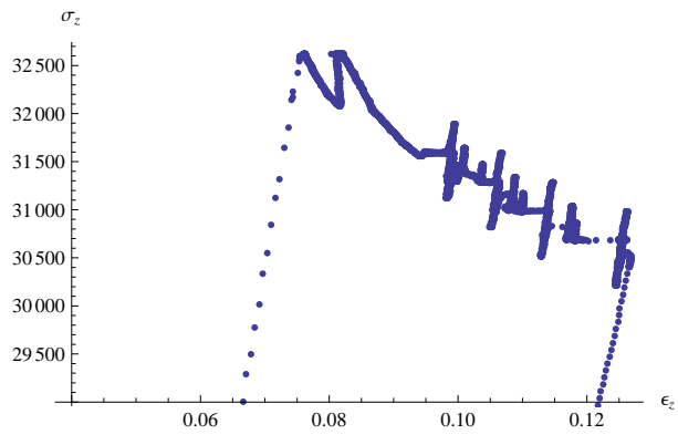
Figure A.28. The \sigma_z/\epsilon_z stress strain plot for test LP-TA23.
