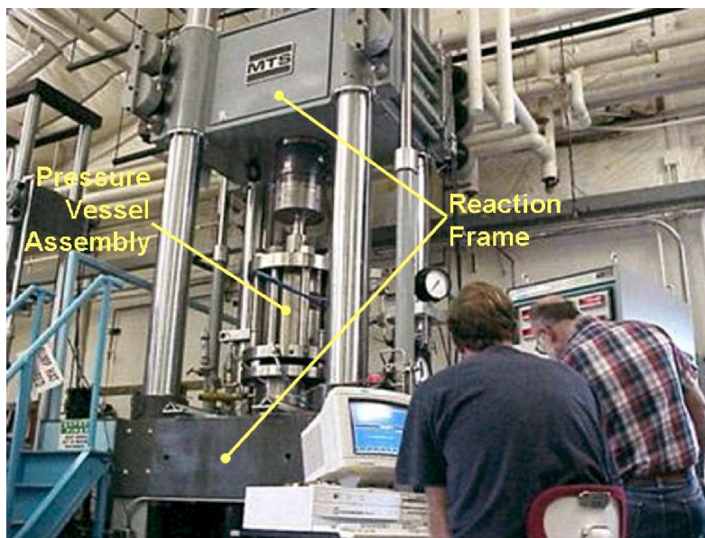
Figure 5.5. Testing system used to conduct quasi-static triaxial compression tests.
