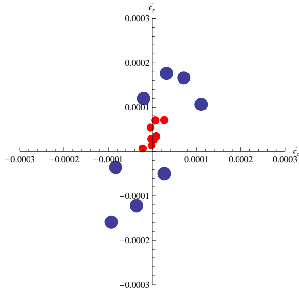
Figure A.57. Strain response envelope for the third loading cycle of test CG2-LP03.
