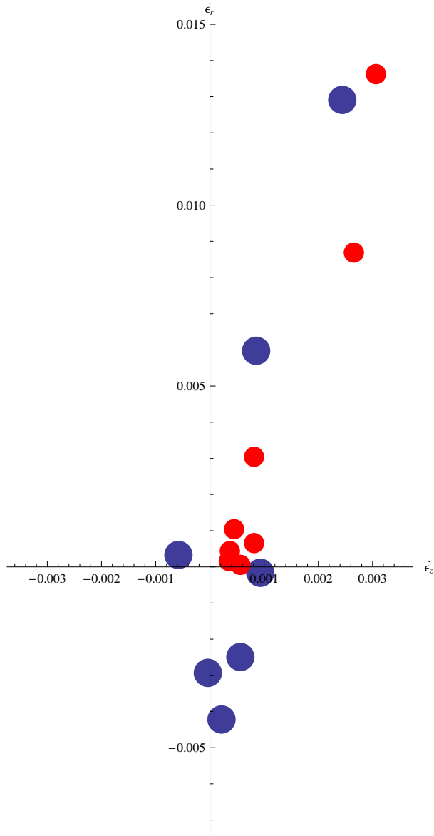
Figure A.29. Strain response envelope for the second loading cycle for test LP-TA23.
