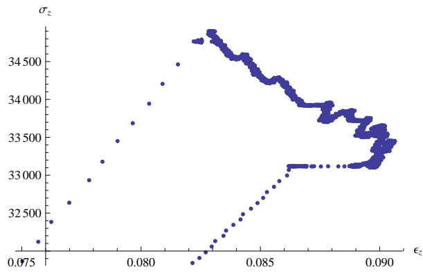
Figure A.11. The \sigma_z/\varepsilon_z stress strain plot for test LP-TA19.
