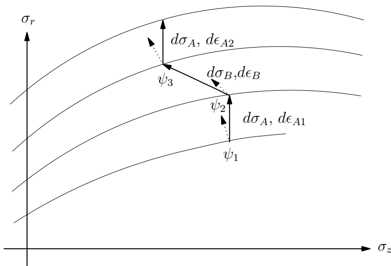
Figure 4.1. A simple cyclically applied incremental loading. Solid vector lines indicate stress vectors, dotted vector lines indicate strain vectors.
