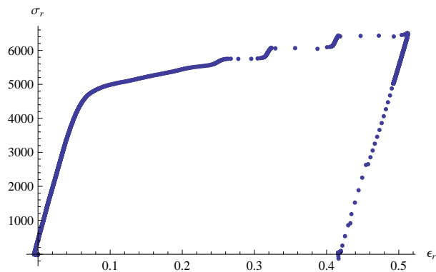
Figure A.39. The \sigma_r/\epsilon_r stress strain plot for test LP-TA25.
