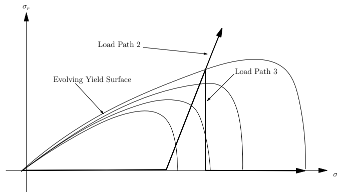
Figure 4.2. Sketch of a triaxial compression test (bold arrow) with a corresponding unvalidated yield surface evolution that predicts outward motion of the cap even after onset of dilatation; in the theoretical model under investigation, the onset of dilatation corresponds to the point where the load path crosses over the peak point of the evolving cap.
