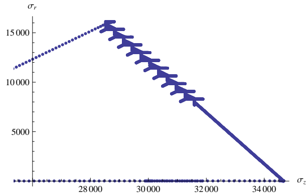
Figure A.53. The loading path used for test CG2-LP03
