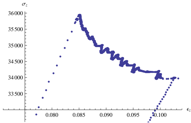
Figure A.18. The \sigma_z/\epsilon_z stress strain plot for test LP-TA21.
