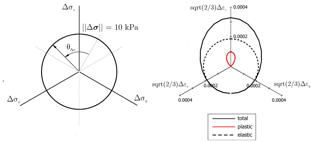
Figure 2.5. Results of Tamagnini's DEM stress probe simulations. A set of deviatoric stress increments represented by a unit circle in stress space (left), and the resulting strain increments mapped to strain space (right). (Courtesy of C. Tamagnini)
