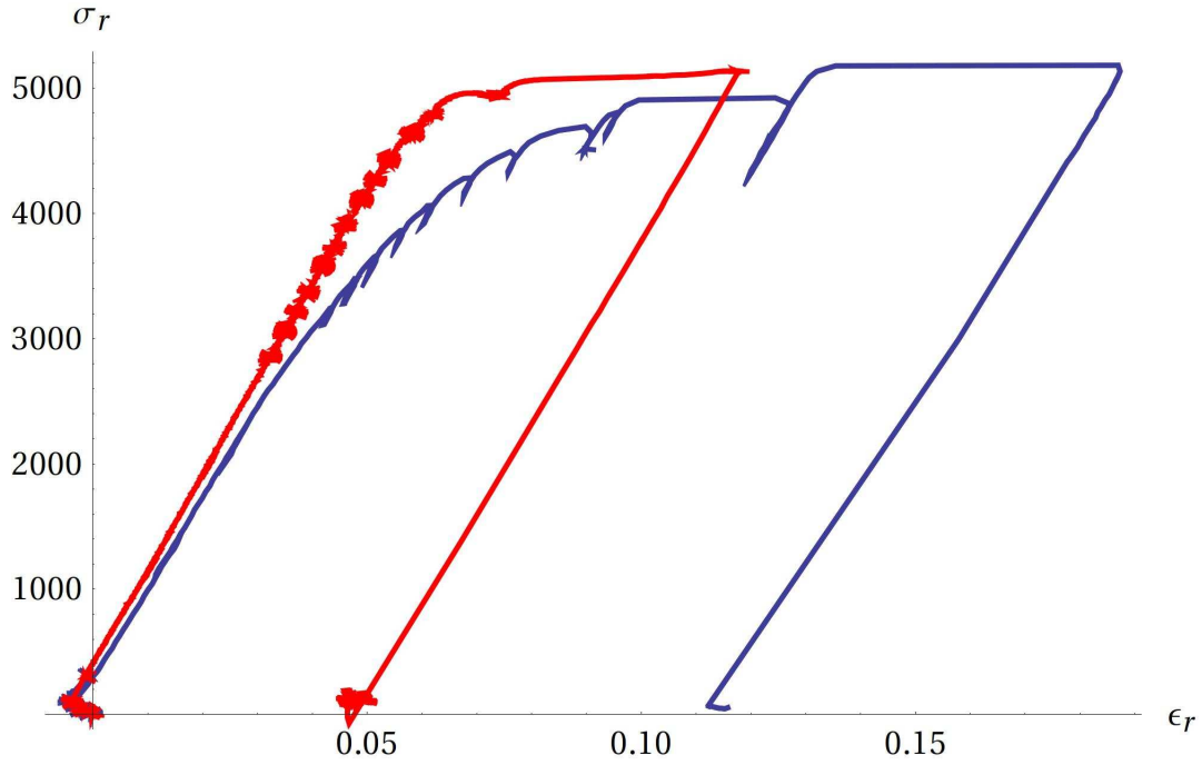
Figure A.12. Equivalent shear stress \sigma_r versus equivalent shear strain \varepsilon_r for test LP-TA18 (blue) and LP-TA19 (red).
